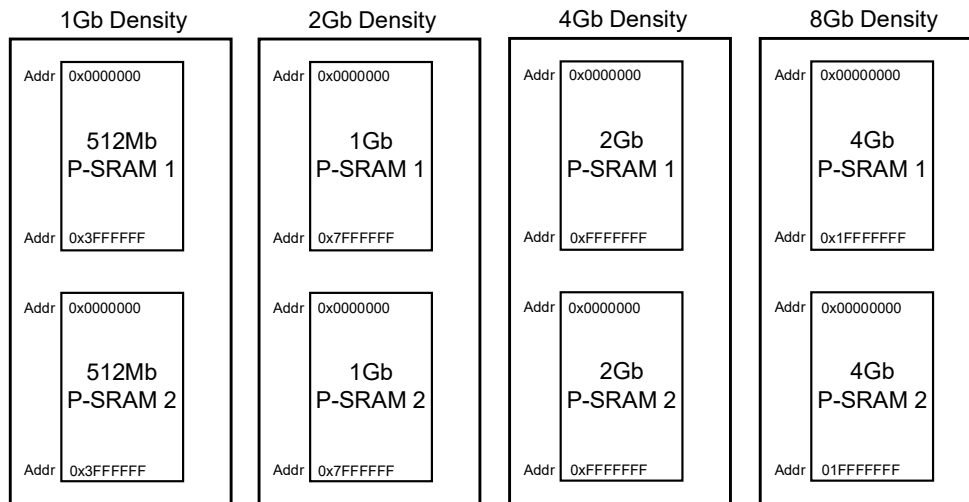
Figure 12: Address Range
