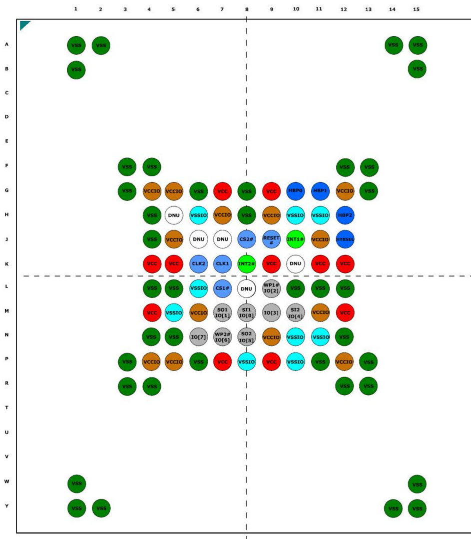
Figure 6: 96-ball FBGA
