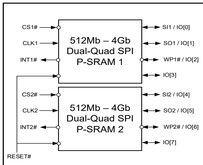
Figure 3: Device Pinout
