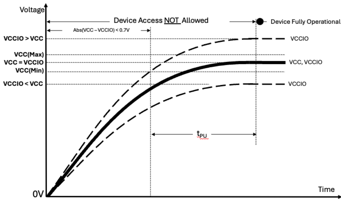
Figure 9: Power-Up Behavior
