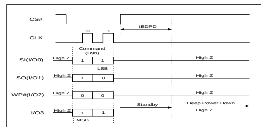
Figure 40: Enter Deep Power Down in QPI Command Sequence
