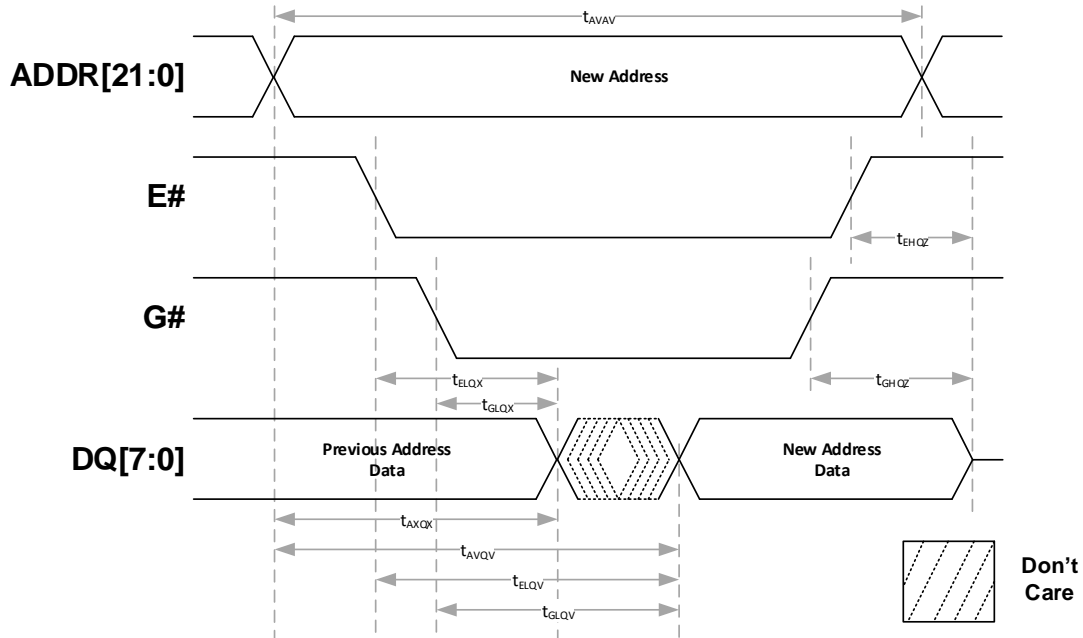
Figure 9: Read Operation
