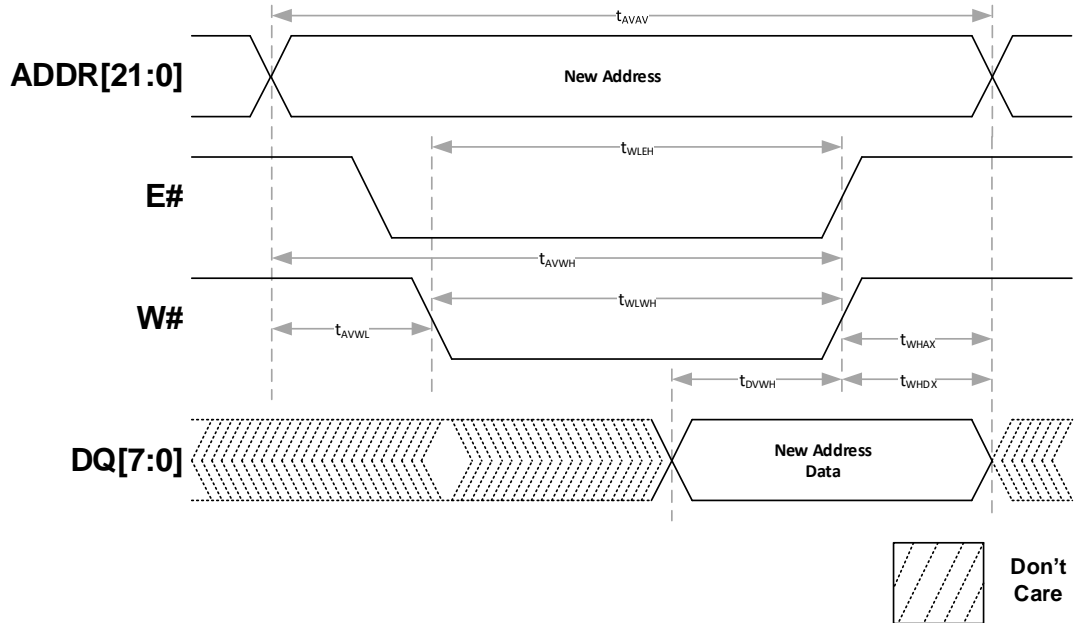
Figure 7: Write Operation
