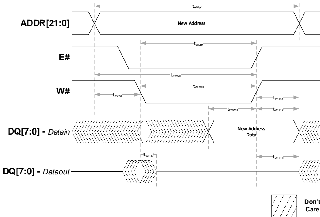
Figure 8: Bus Turnaround Operation
