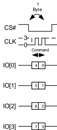
Figure 17: Description of (4-0-0) Instruction Type
