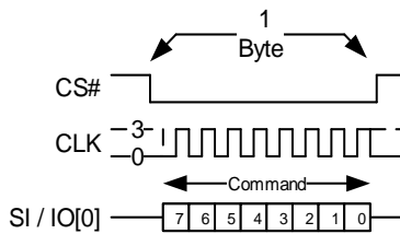
Figure 11: Description of (1-0-0) Instruction Type
